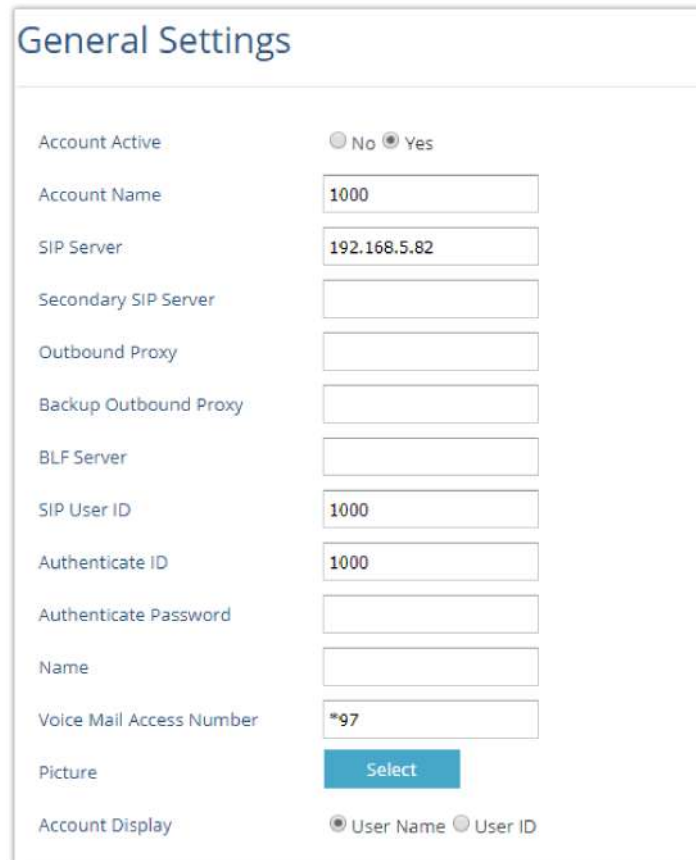
Figure 47: Web UI – Voice Mail Access Number
