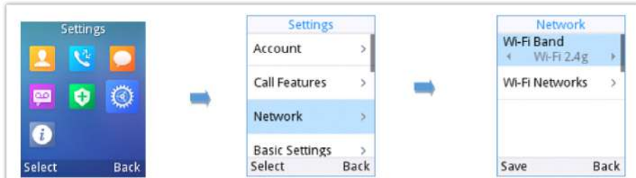
Figure 19: Wi-Fi Band Configuration
